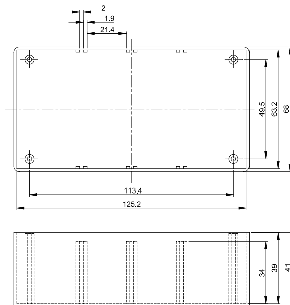
G1022B
