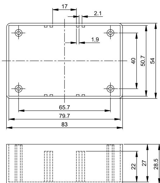
G1020B
