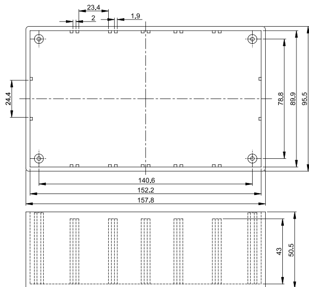
G1024B
